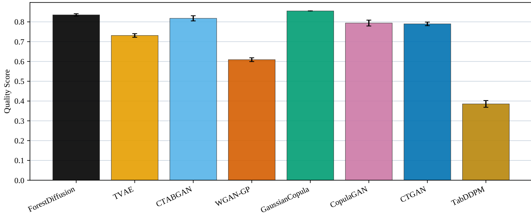
Bank Marketing — Quality Score (mean \pm SD, 10 seeds)
